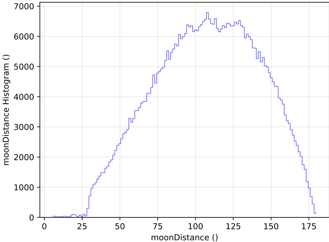
too_elab_r8_d2_gz_v3.4_10yrs All sky r band: moonDistance Histogram
