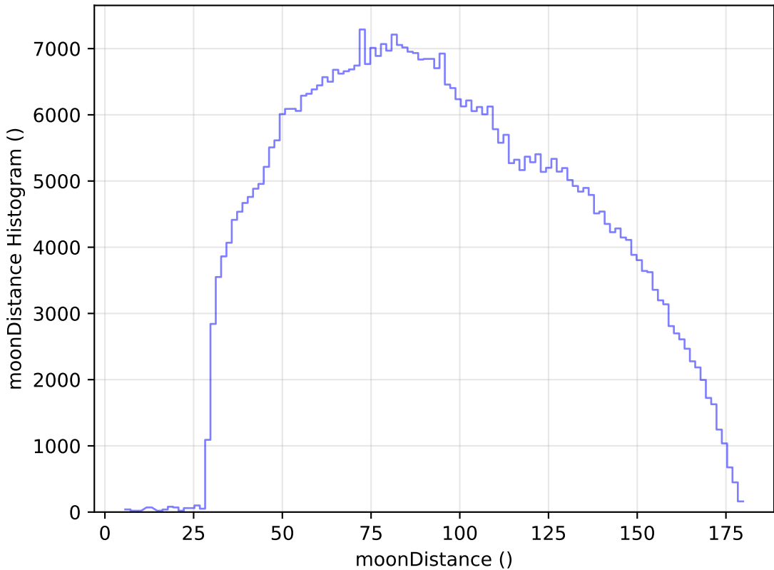
too_elab_r8_d2_gz_v3.4_10yrs All sky i band: moonDistance Histogram
