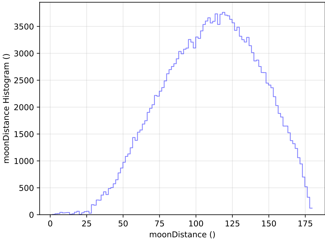
too_elab_r8_d2_gz_v3.4_10yrs All sky g band: moonDistance Histogram
