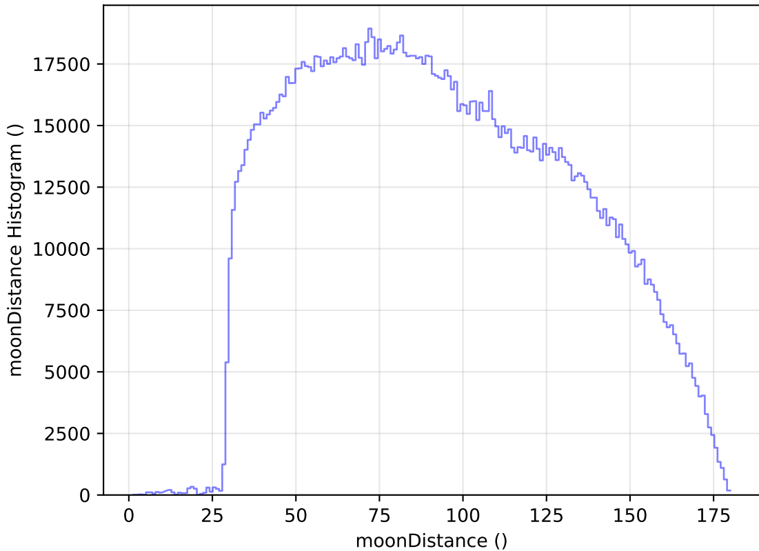
too_elab_r8_d2_gz_v3.4_10yrs All sky all bands: moonDistance Histogram
