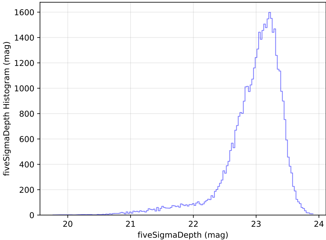
too_elab_r8_d2_gz_v3.4_10yrs Yr 1 z band: fiveSigmaDepth Histogram
