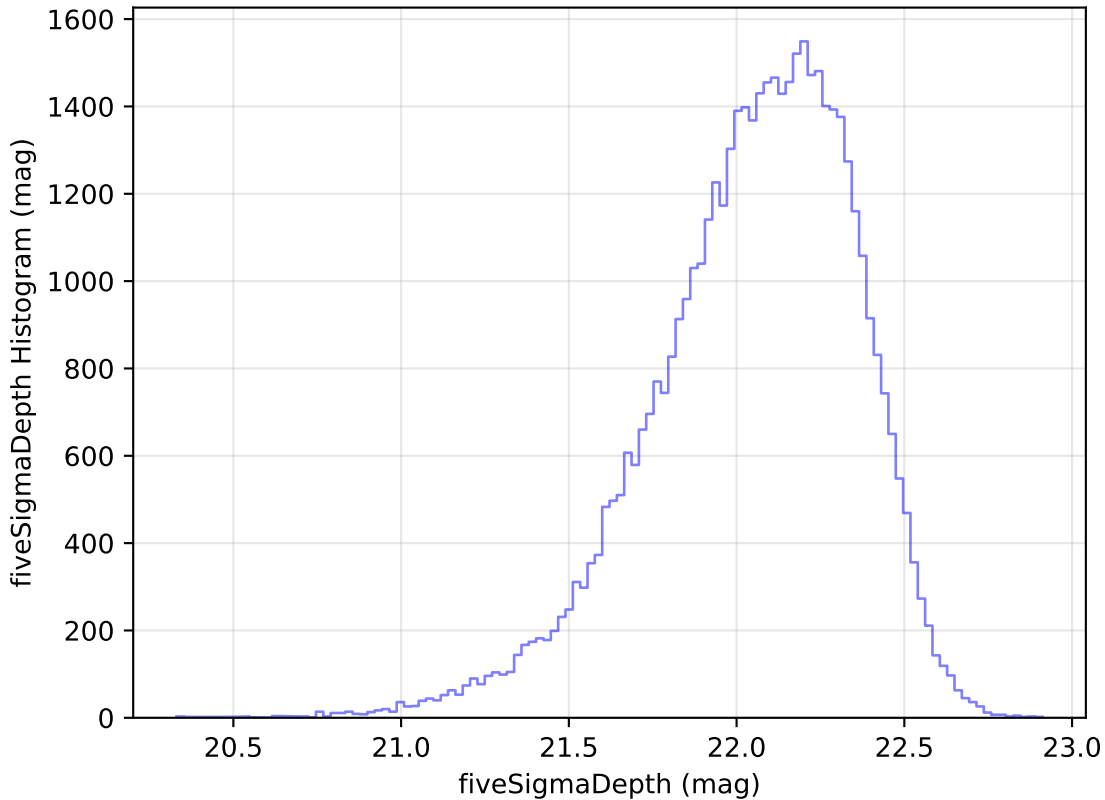
too_elab_r8_d2_gz_v3.4_10yrs Yr 1 y band: fiveSigmaDepth Histogram
