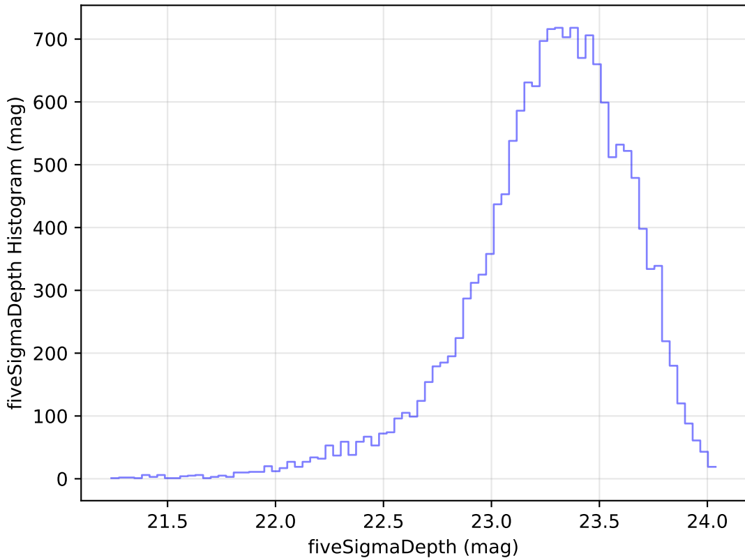
too_elab_r8_d2_gz_v3.4_10yrs Yr 1 u band: fiveSigmaDepth Histogram
