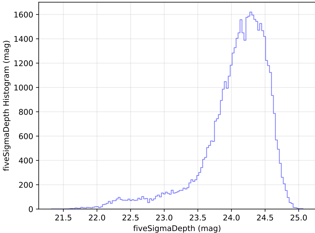
too_elab_r8_d2_gz_v3.4_10yrs Yr 1 r band: fiveSigmaDepth Histogram
