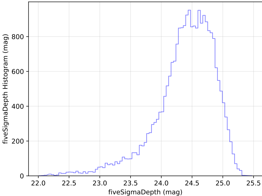
too_elab_r8_d2_gz_v3.4_10yrs Yr 1 g band: fiveSigmaDepth Histogram
