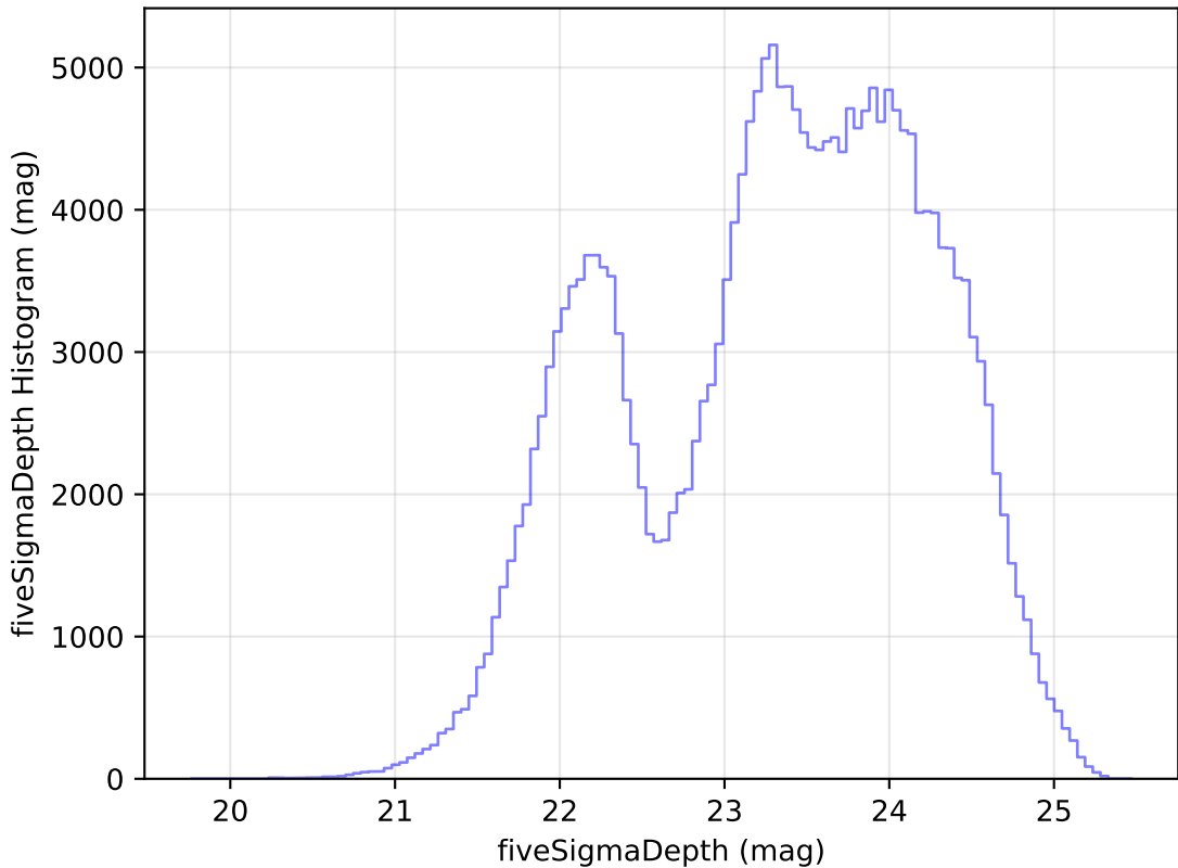
too_elab_r8_d2_gz_v3.4_10yrs Yr 1 all bands: fiveSigmaDepth Histogram
