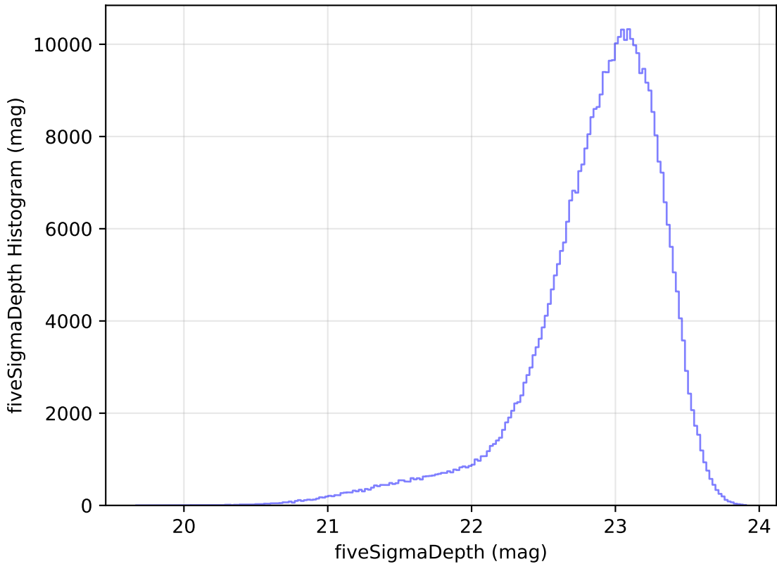
too_elab_r8_d2_gz_v3.4_10yrs WFD z band: fiveSigmaDepth Histogram
