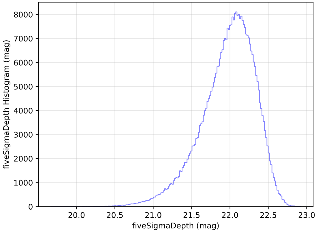
too_elab_r8_d2_gz_v3.4_10yrs WFD y band: fiveSigmaDepth Histogram
