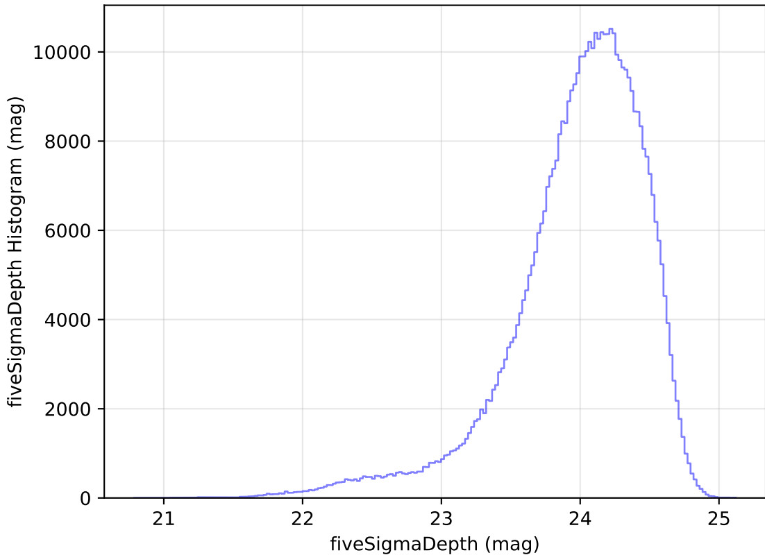
too_elab_r8_d2_gz_v3.4_10yrs WFD r band: fiveSigmaDepth Histogram
