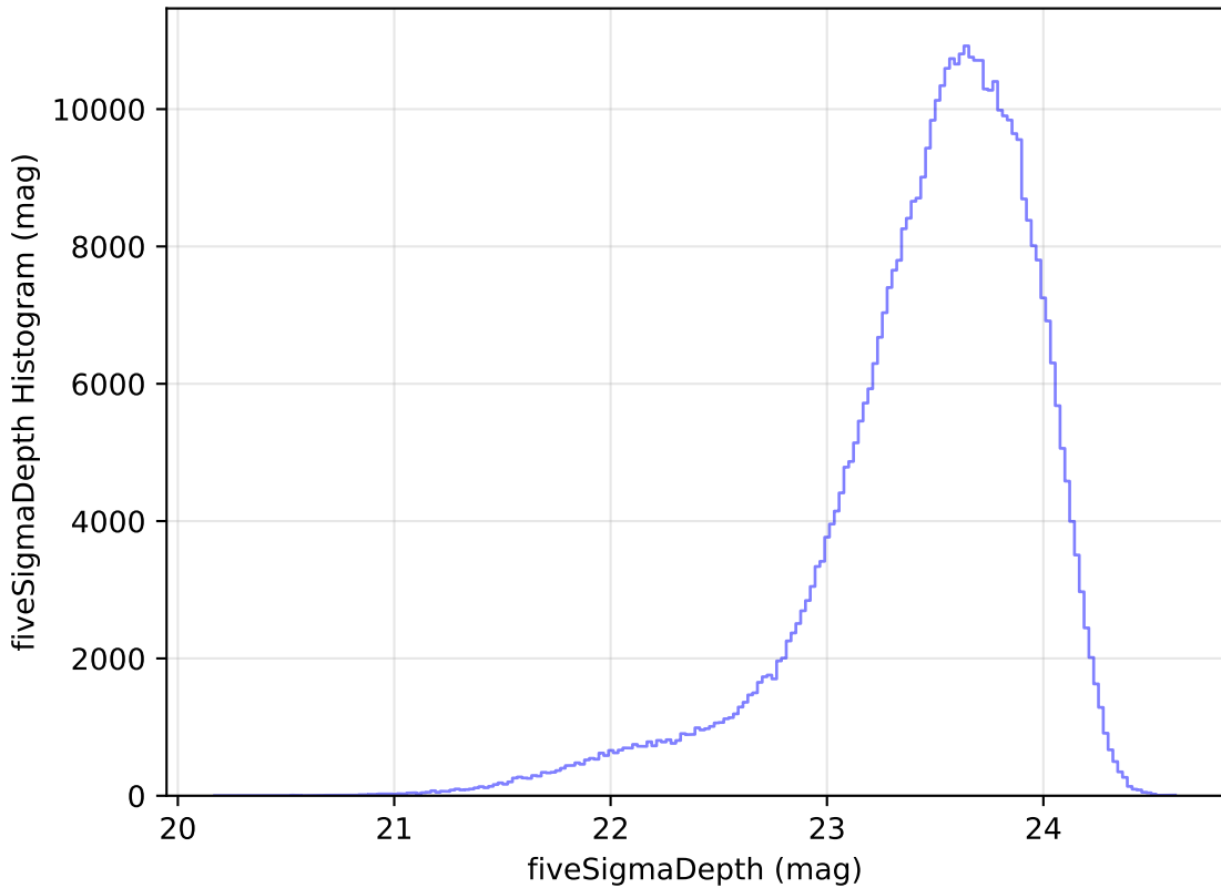
too_elab_r8_d2_gz_v3.4_10yrs WFD i band: fiveSigmaDepth Histogram
