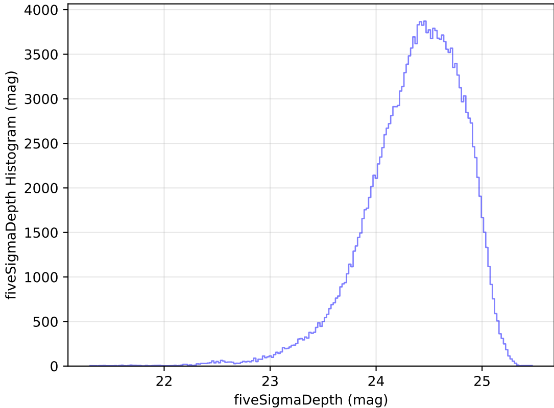
too_elab_r8_d2_gz_v3.4_10yrs WFD g band: fiveSigmaDepth Histogram
