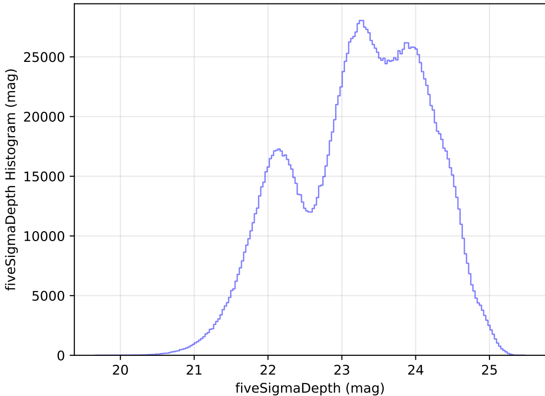
too_elab_r8_d2_gz_v3.4_10yrs WFD all bands: fiveSigmaDepth Histogram
