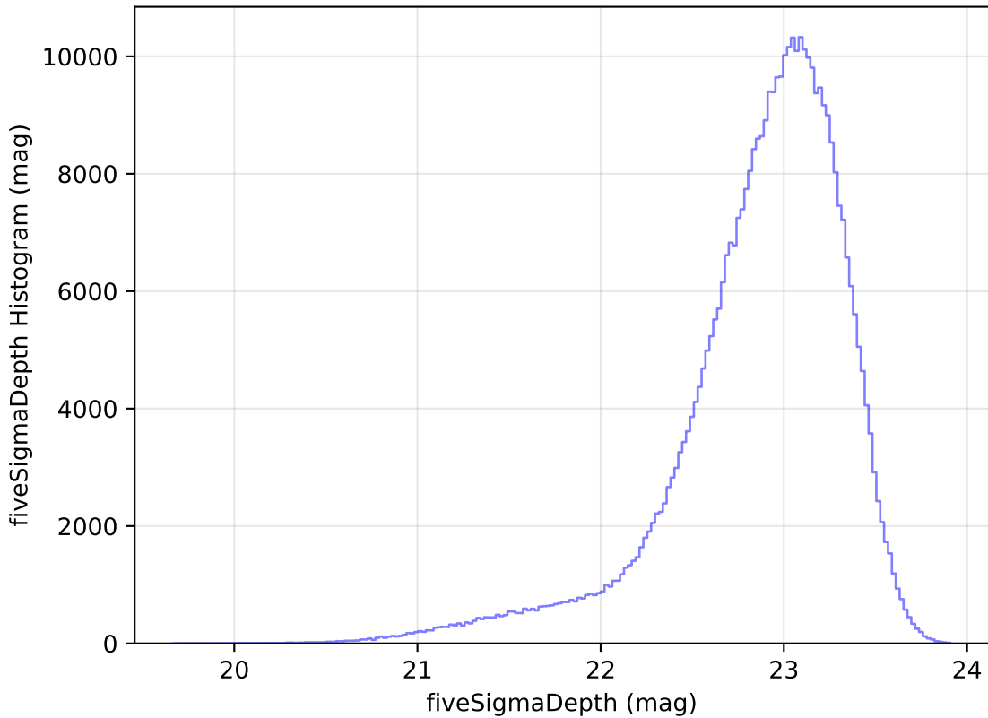
too_elab_r8_d2_gz_v3.4_10yrs All sky z band: fiveSigmaDepth Histogram
