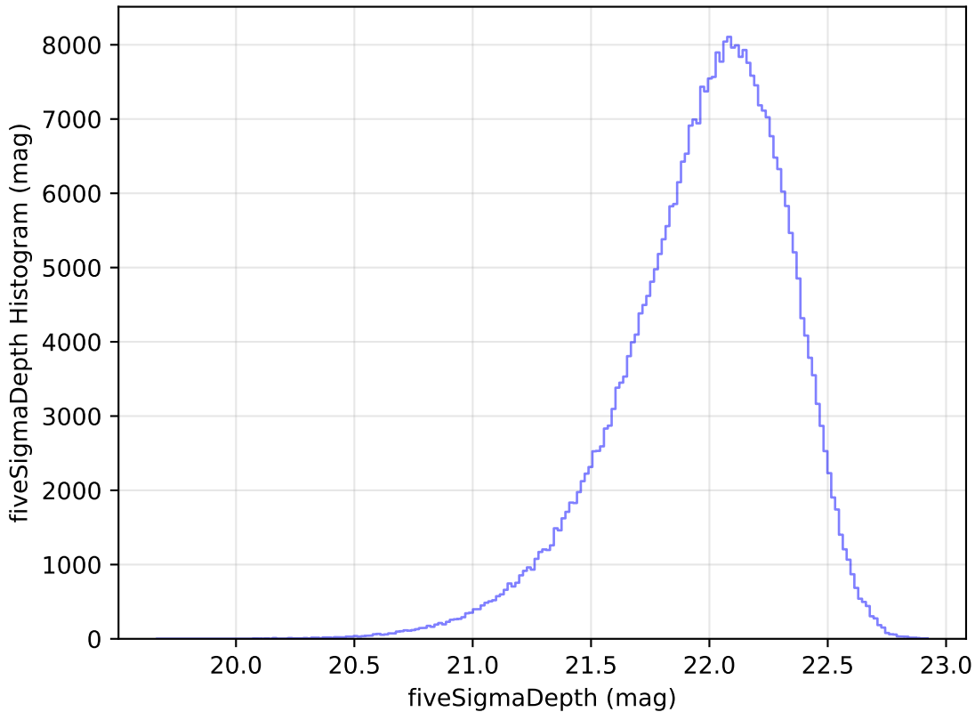
too_elab_r8_d2_gz_v3.4_10yrs All sky y band: fiveSigmaDepth Histogram
