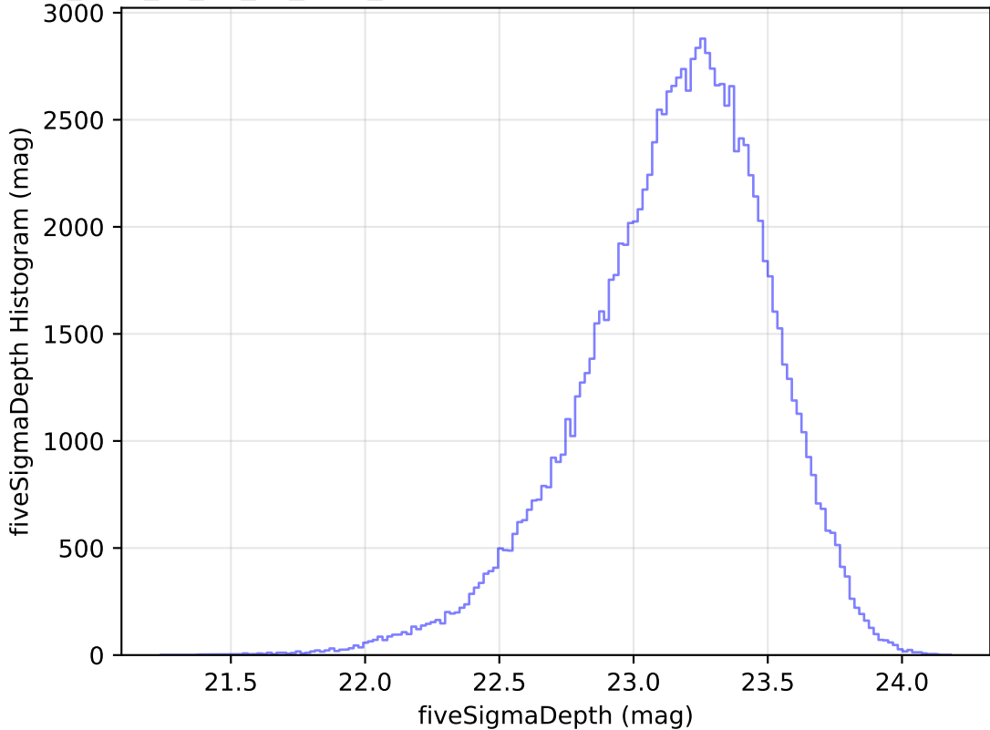
too_elab_r8_d2_gz_v3.4_10yrs All sky u band: fiveSigmaDepth Histogram
