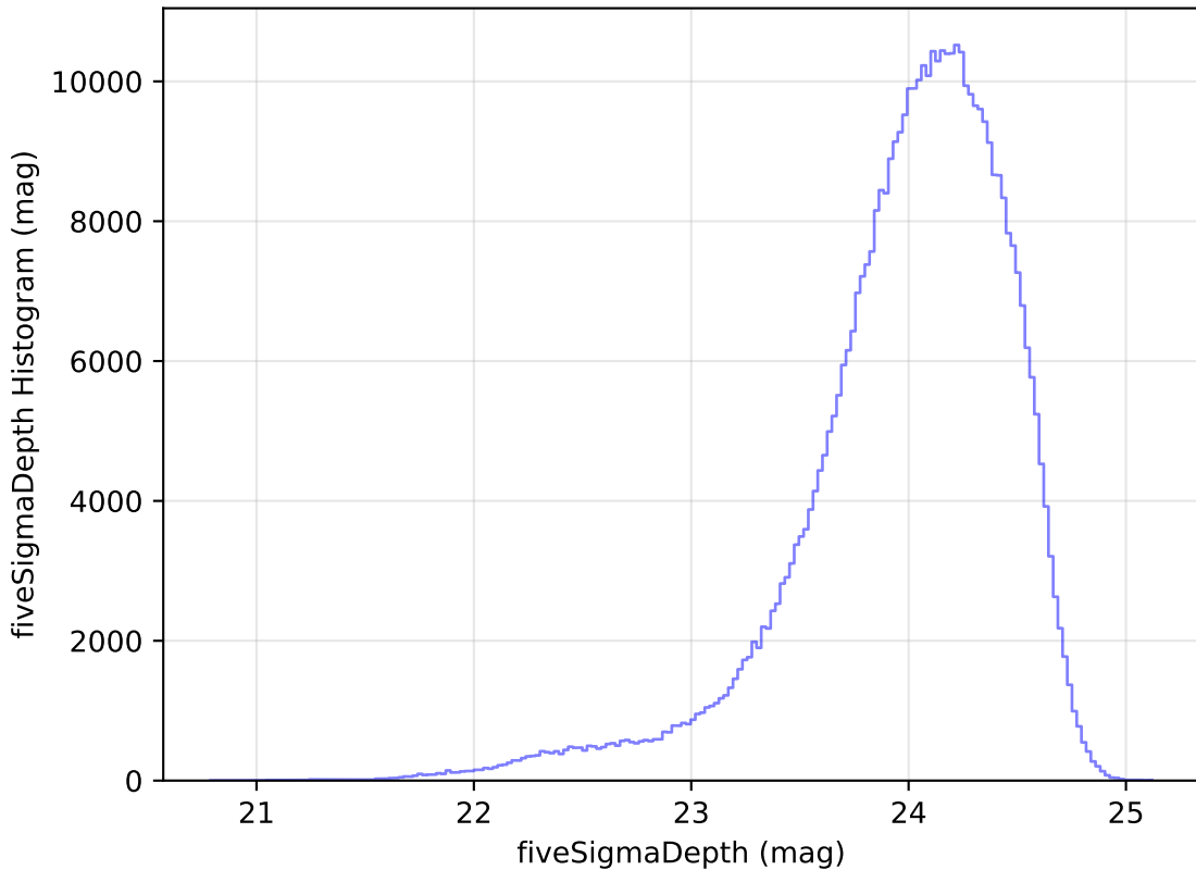
too_elab_r8_d2_gz_v3.4_10yrs All sky r band: fiveSigmaDepth Histogram
