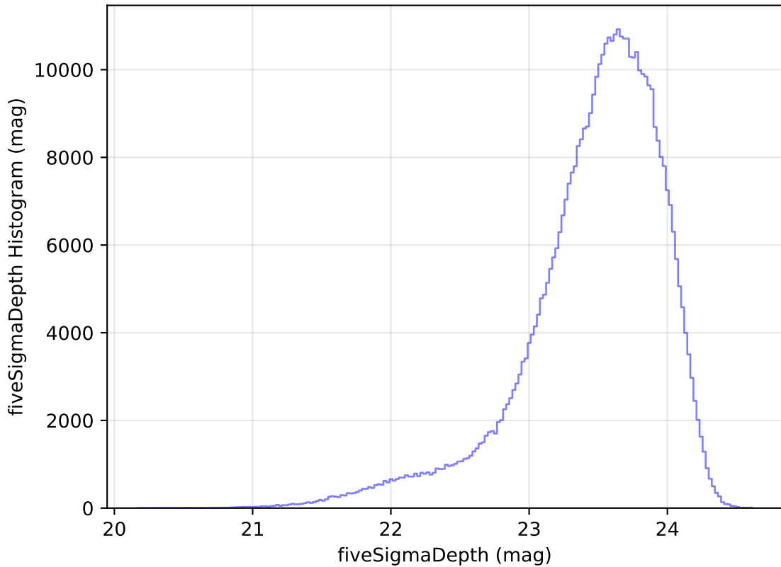
too_elab_r8_d2_gz_v3.4_10yrs All sky i band: fiveSigmaDepth Histogram
