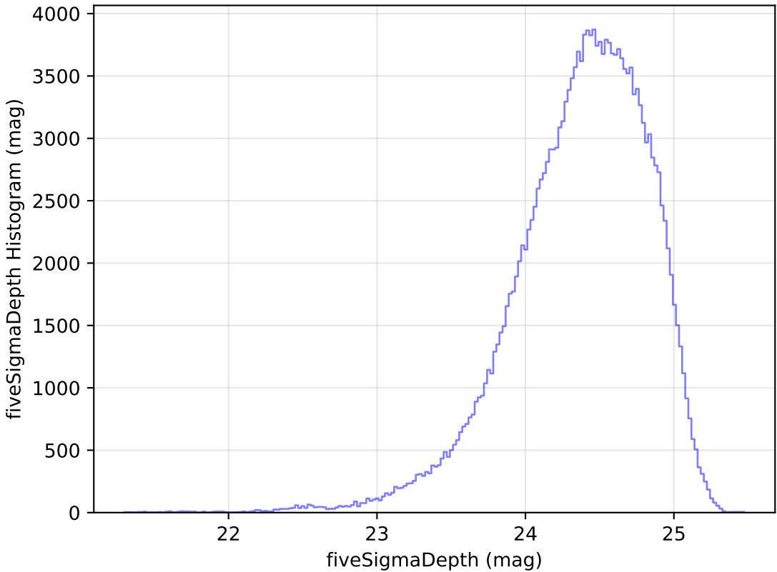
too_elab_r8_d2_gz_v3.4_10yrs All sky g band: fiveSigmaDepth Histogram
