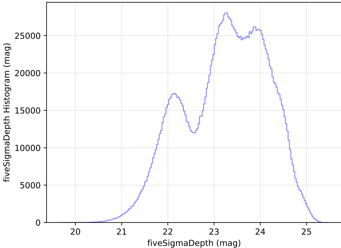
too_elab_r8_d2_gz_v3.4_10yrs All sky all bands: fiveSigmaDepth Histogram
