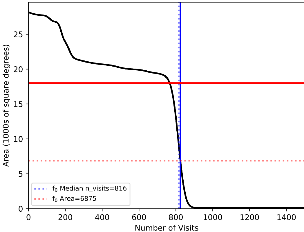
too_elab_r8_d2_gz_v3.4_10yrs All sky: f0
