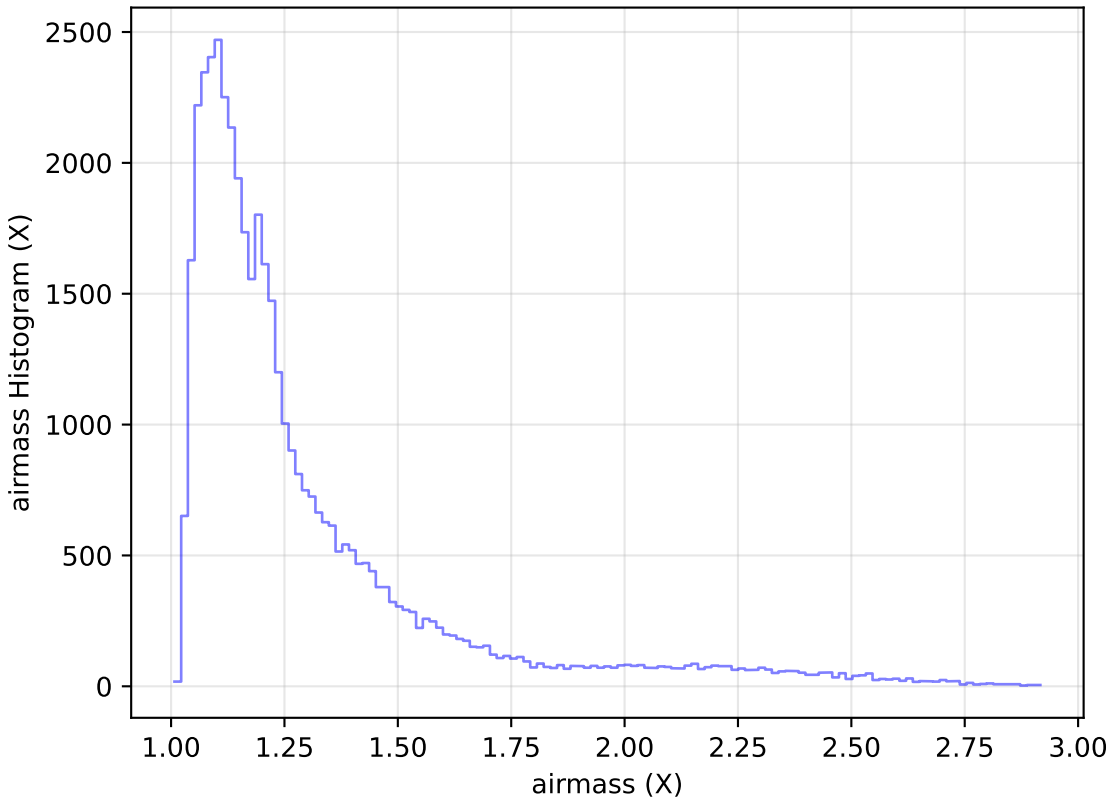
too_elab_r8_d2_gz_v3.4_10yrs Yr 1 z band: airmass Histogram
