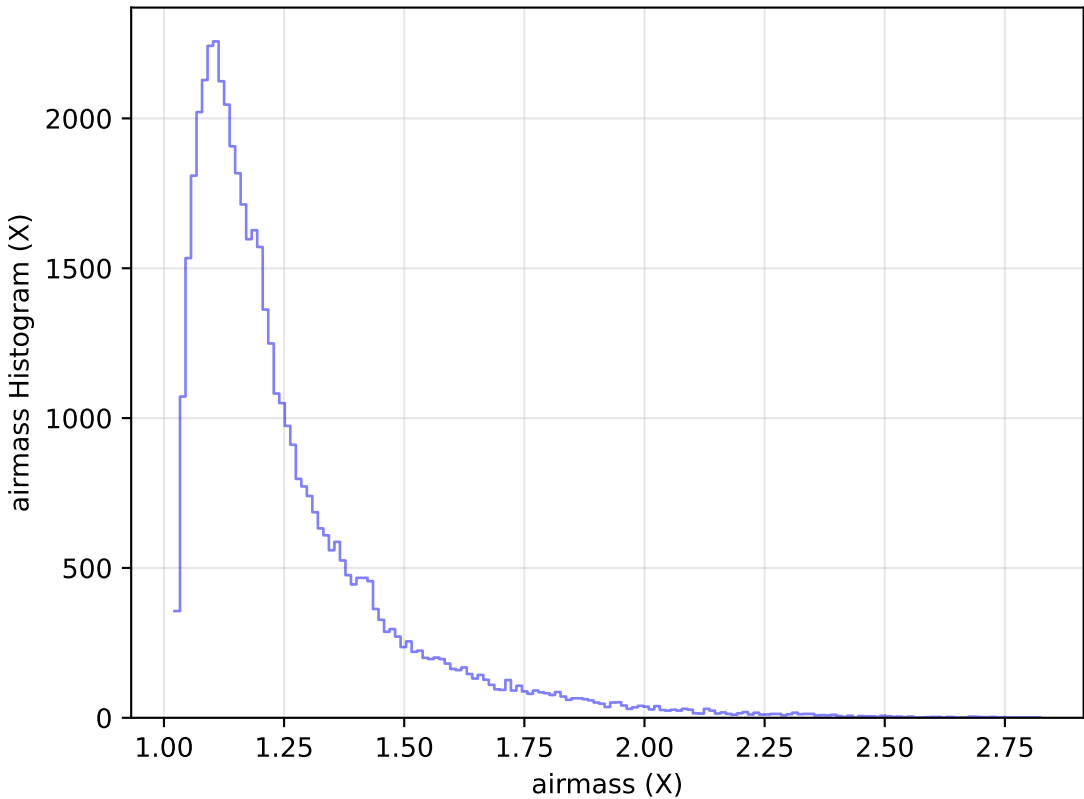
too_elab_r8_d2_gz_v3.4_10yrs Yr 1 y band: airmass Histogram
