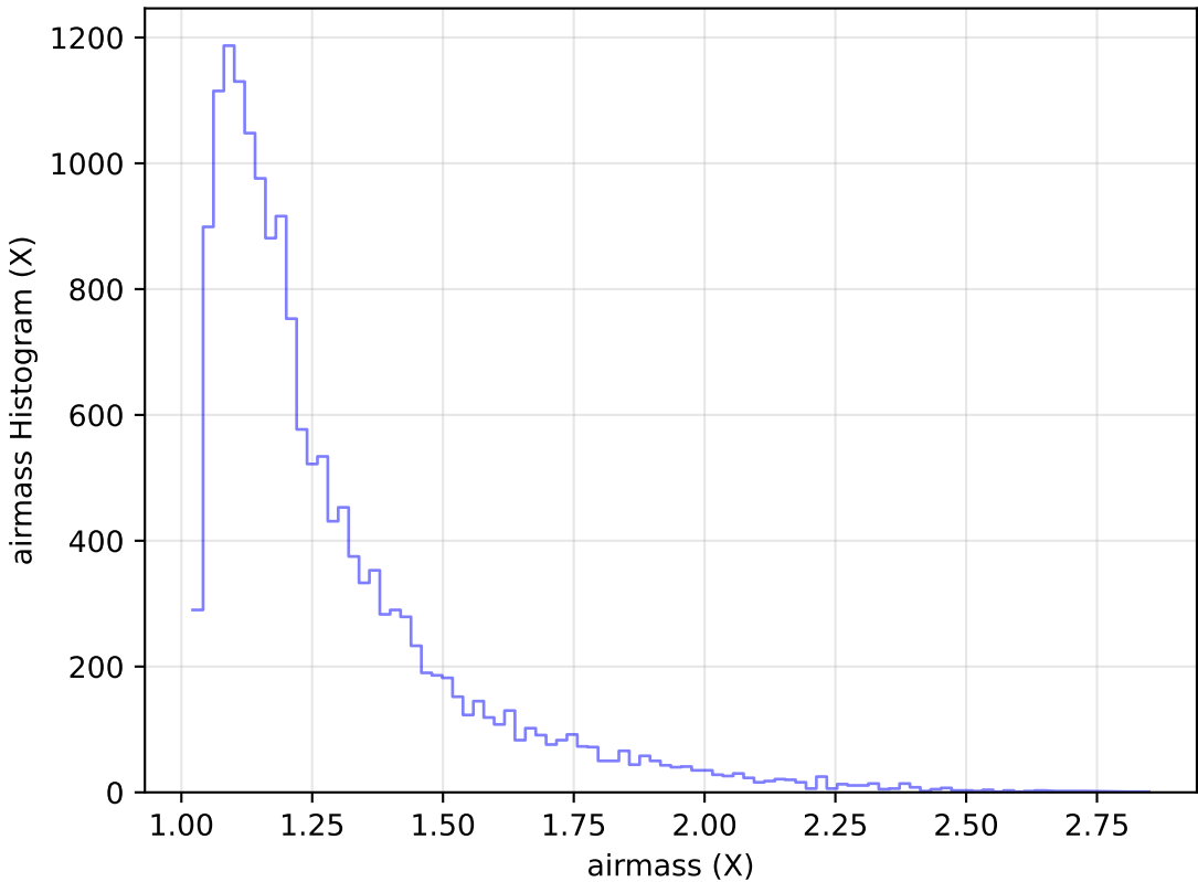
too_elab_r8_d2_gz_v3.4_10yrs Yr 1 u band: airmass Histogram
