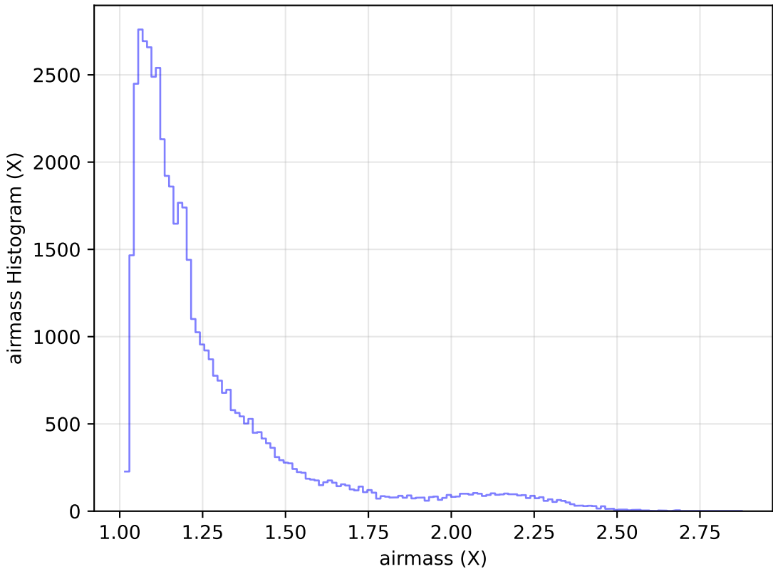
too_elab_r8_d2_gz_v3.4_10yrs Yr 1 r band: airmass Histogram
