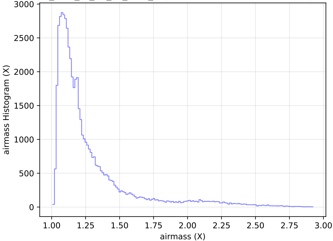
too_elab_r8_d2_gz_v3.4_10yrs Yr 1 i band: airmass Histogram
