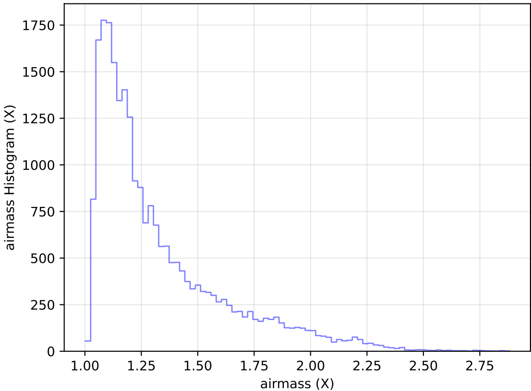
too_elab_r8_d2_gz_v3.4_10yrs Yr 1 g band: airmass Histogram
