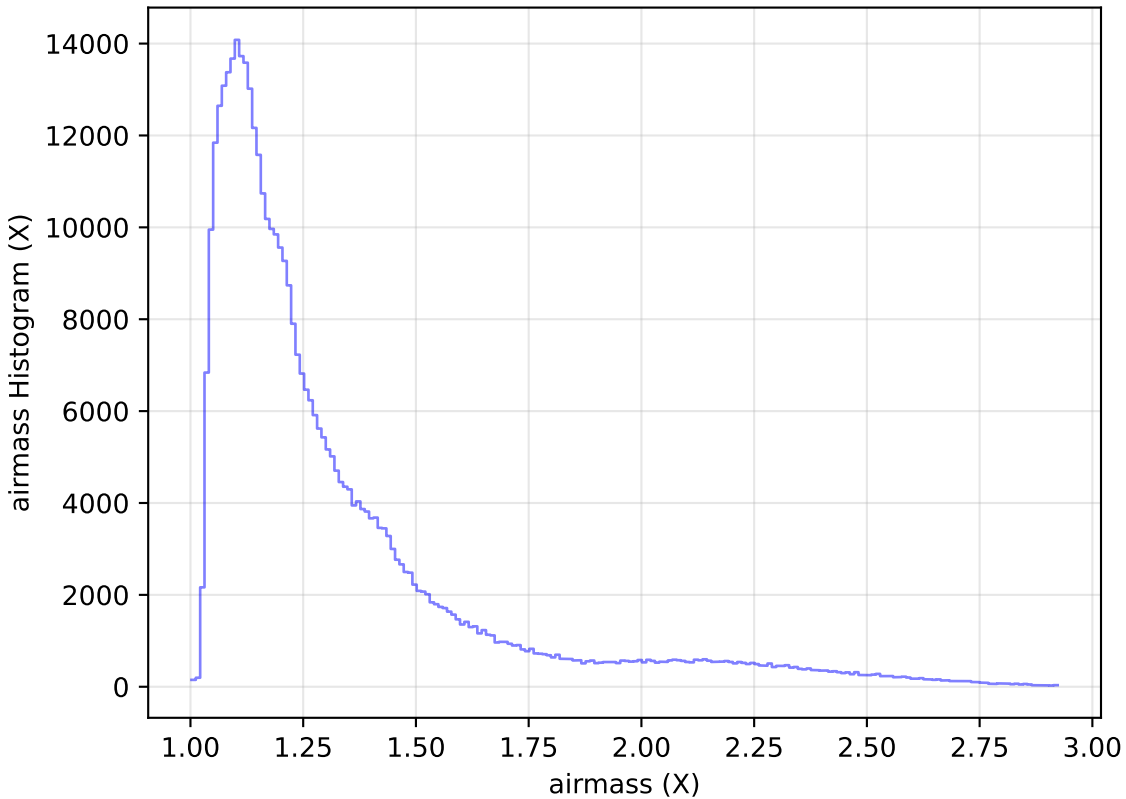
too_elab_r8_d2_gz_v3.4_10yrs WFD z band: airmass Histogram
