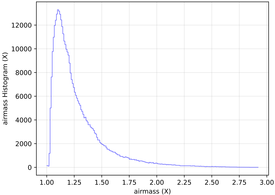
too_elab_r8_d2_gz_v3.4_10yrs WFD y band: airmass Histogram
