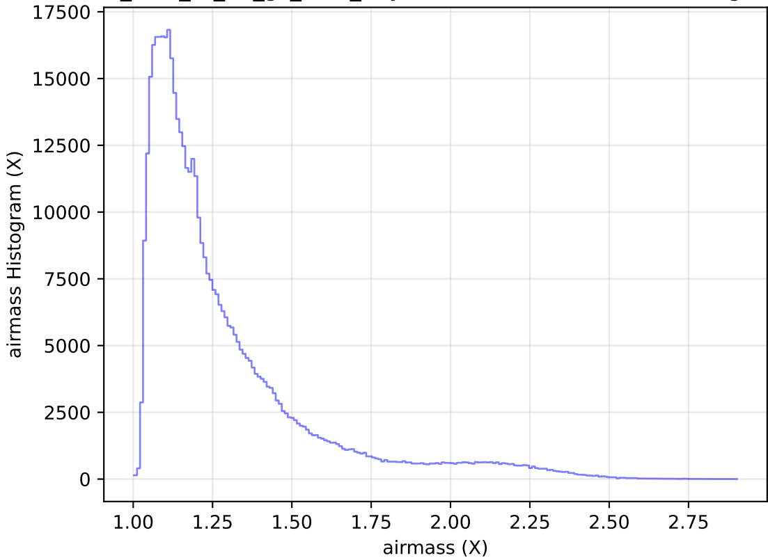
too_elab_r8_d2_gz_v3.4_10yrs WFD r band: airmass Histogram
