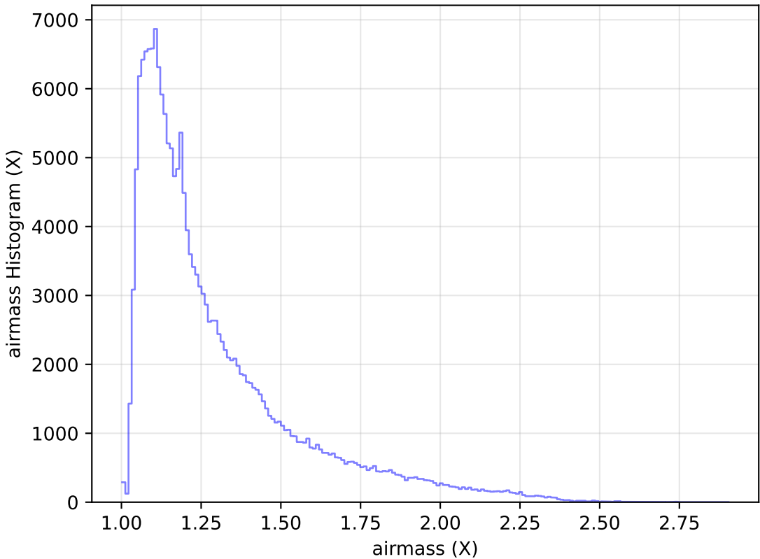
too_elab_r8_d2_gz_v3.4_10yrs WFD g band: airmass Histogram
