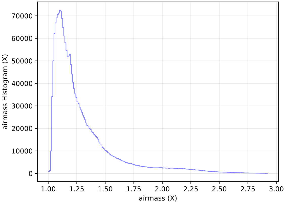
too_elab_r8_d2_gz_v3.4_10yrs WFD all bands: airmass Histogram
