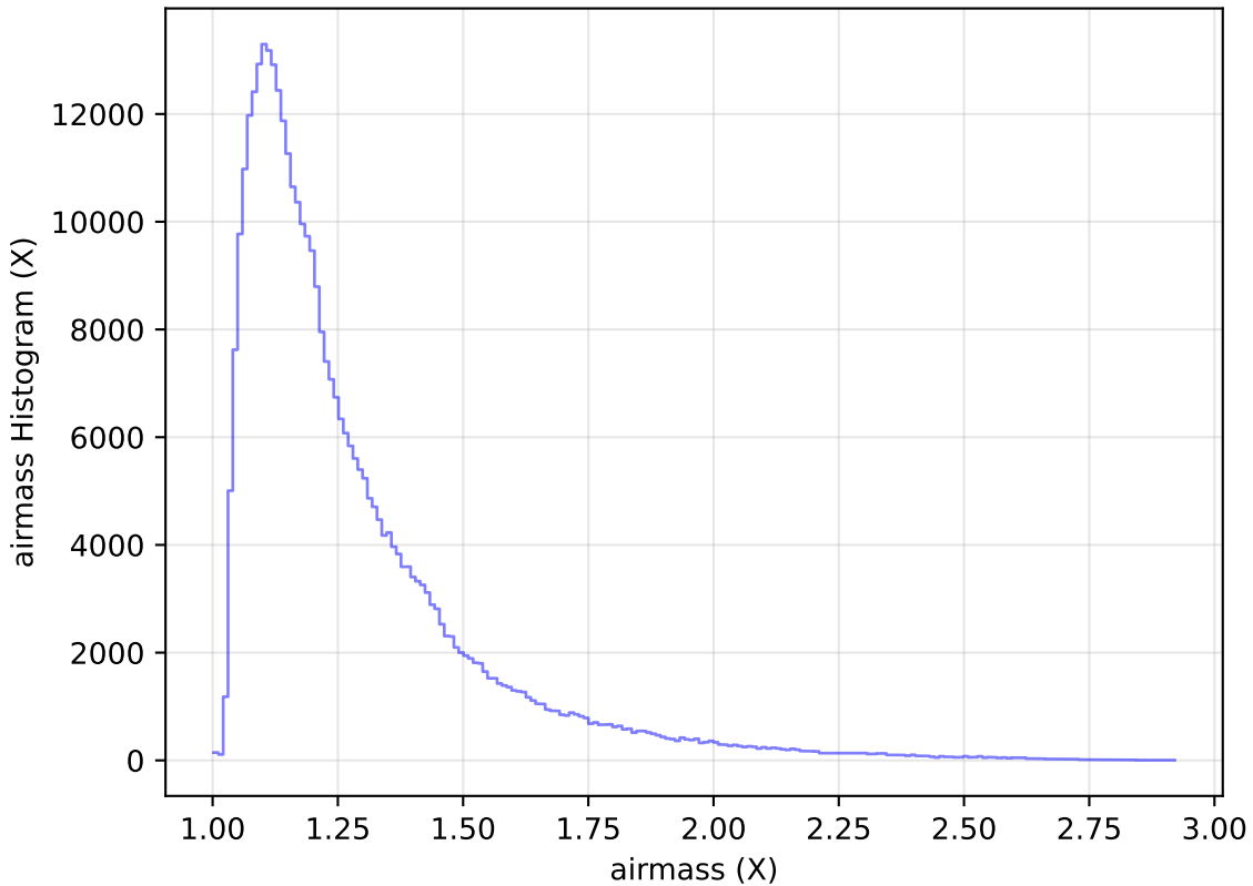
too_elab_r8_d2_gz_v3.4_10yrs All sky y band: airmass Histogram
