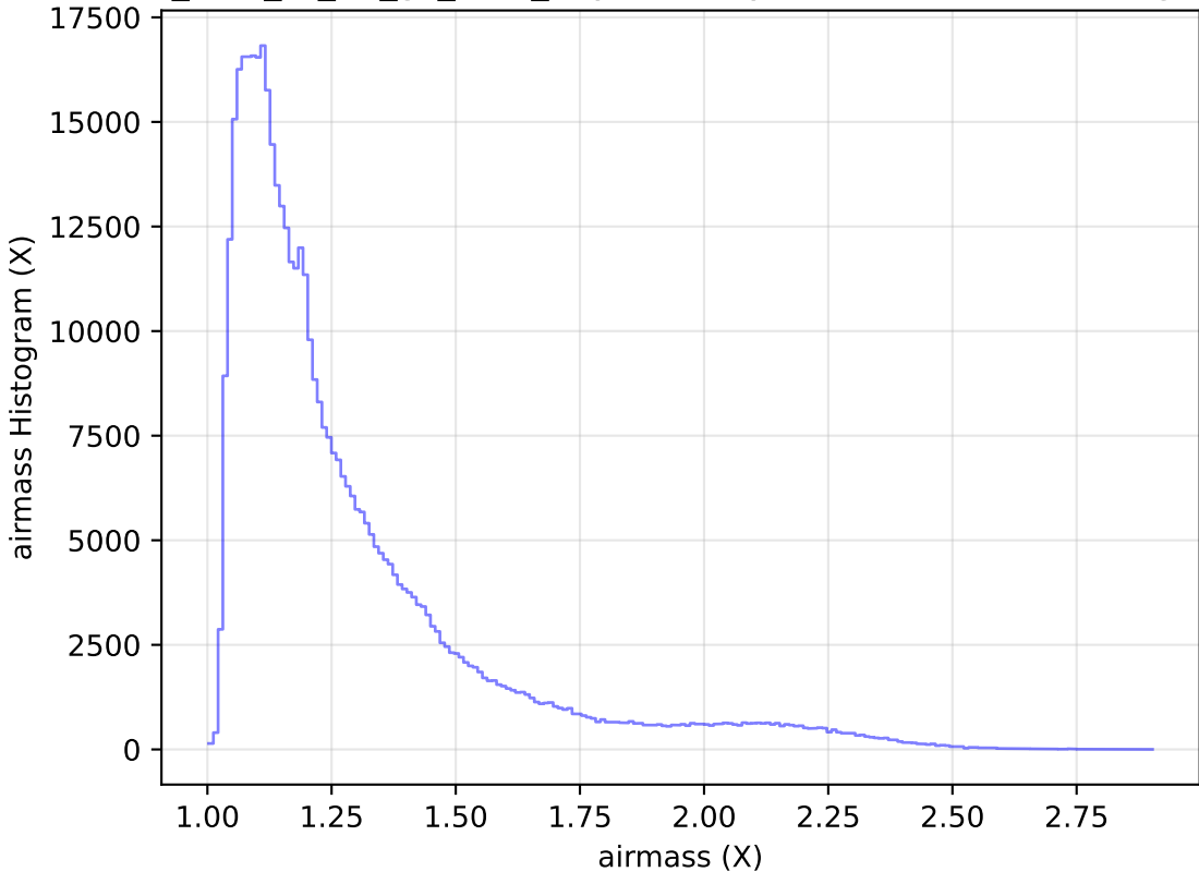
too_elab_r8_d2_gz_v3.4_10yrs All sky r band: airmass Histogram
