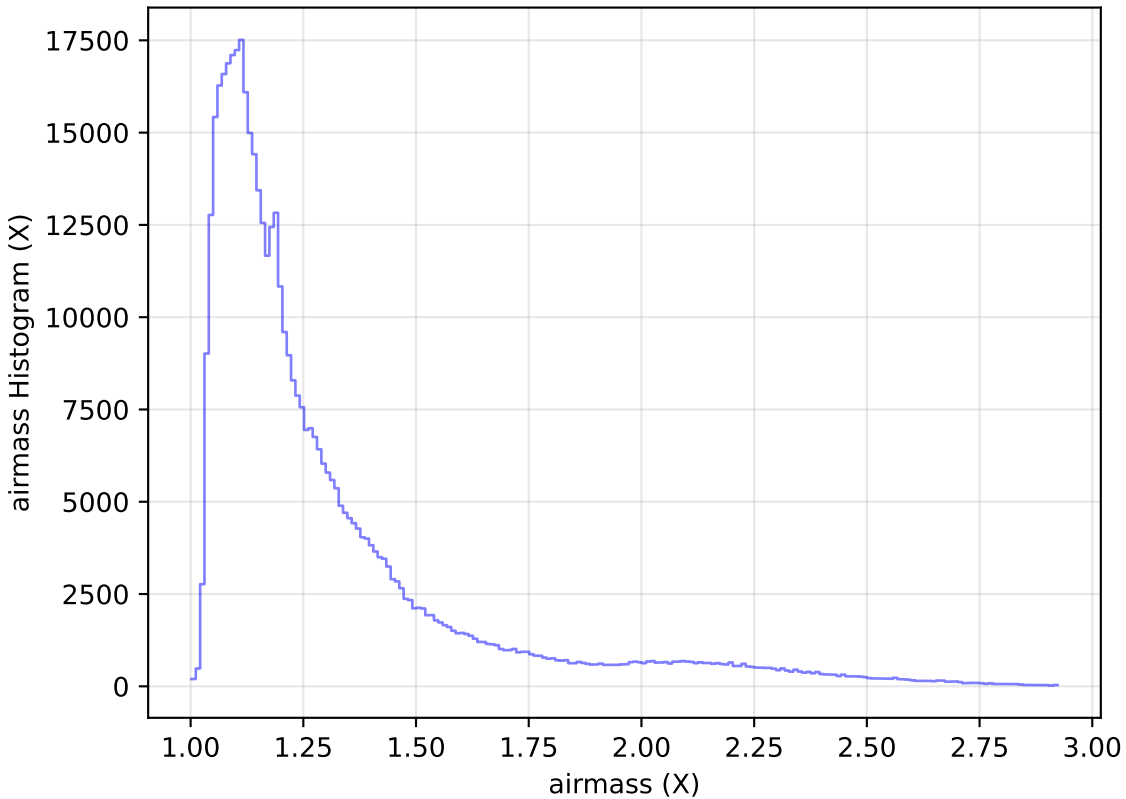
too_elab_r8_d2_gz_v3.4_10yrs All sky i band: airmass Histogram
