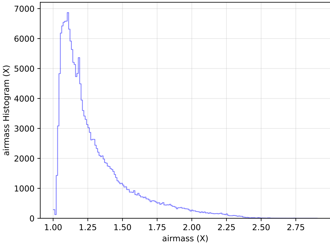
too_elab_r8_d2_gz_v3.4_10yrs All sky g band: airmass Histogram
