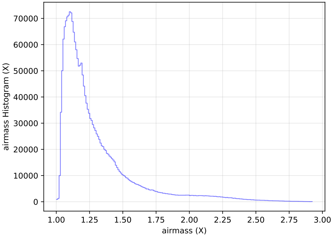
too_elab_r8_d2_gz_v3.4_10yrs All sky all bands: airmass Histogram
