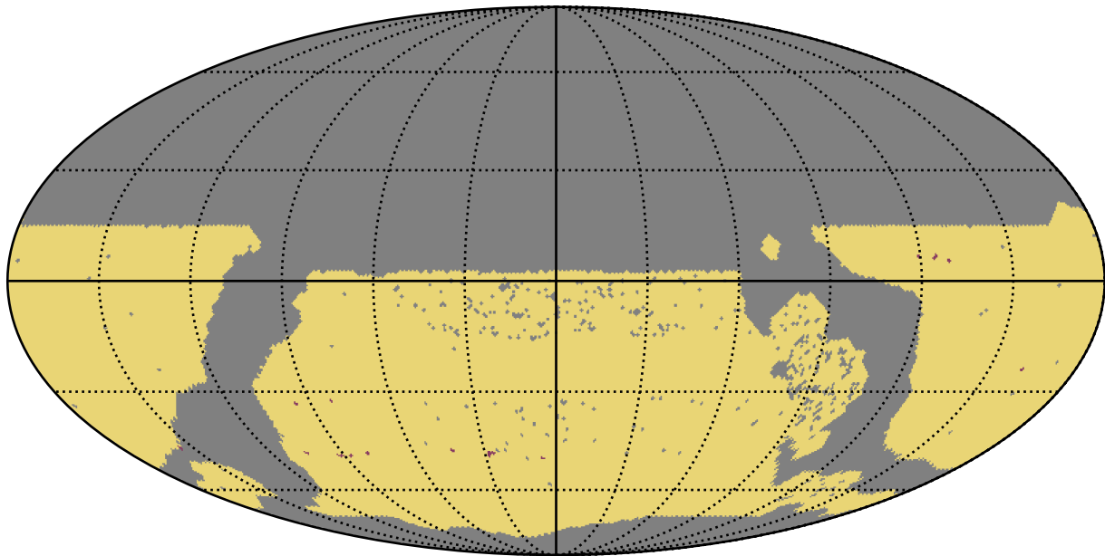
too_elab_r8_d2_gz_v3.4_10yrs WFD: RapidRevisits
