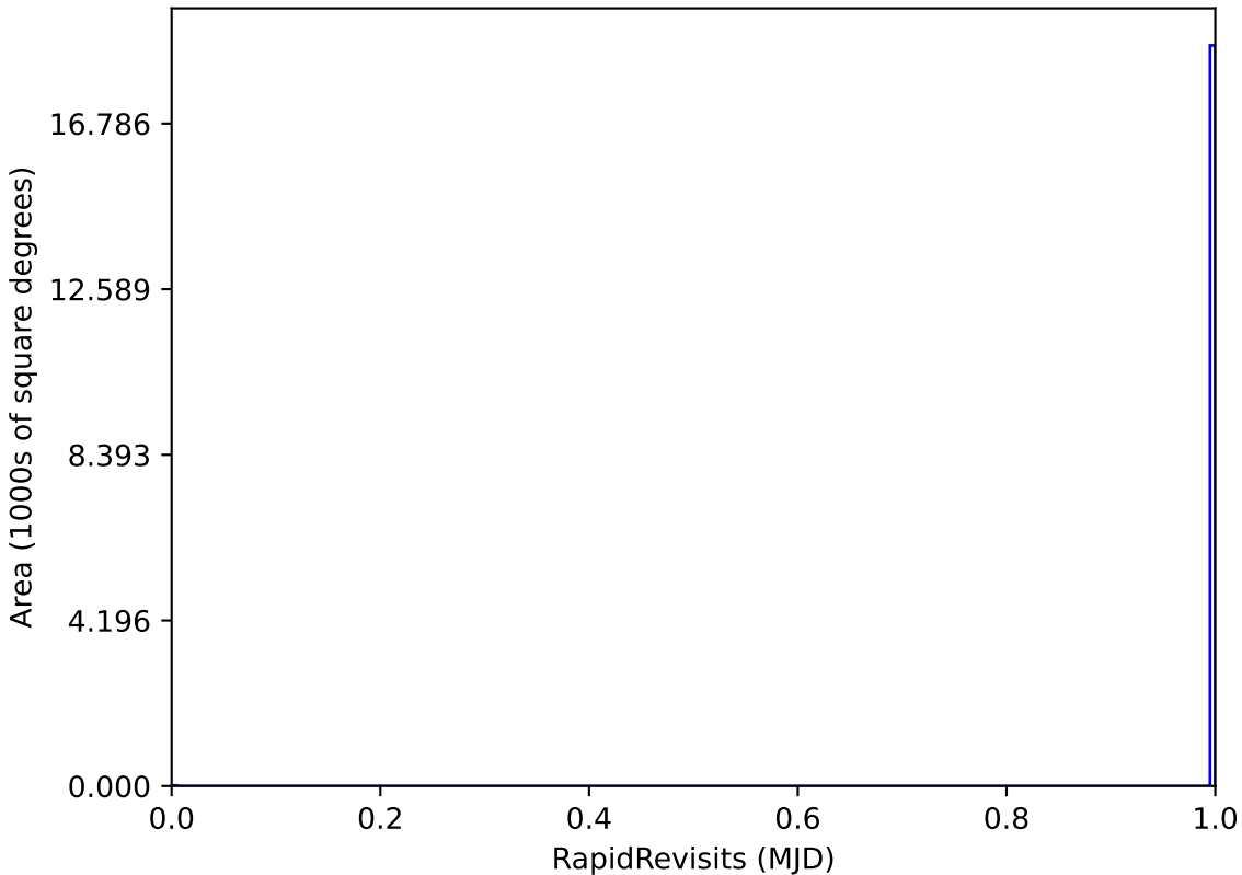
too_elab_r8_d2_gz_v3.4_10yrs WFD: RapidRevisits
