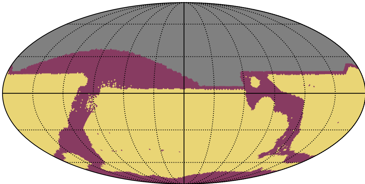
too_elab_r8_d2_gz_v3.4_10yrs All sky: RapidRevisits
