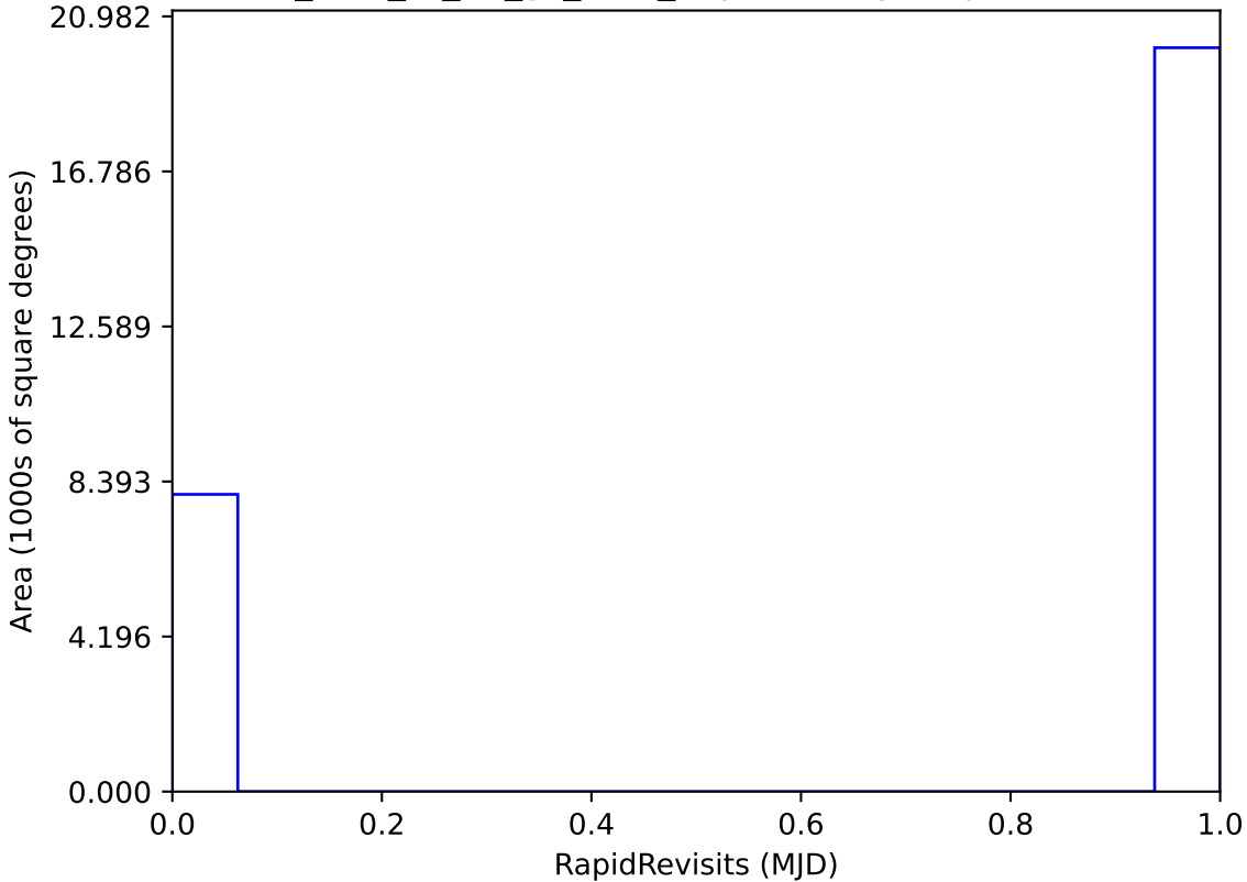
too_elab_r8_d2_gz_v3.4_10yrs All sky: RapidRevisits
