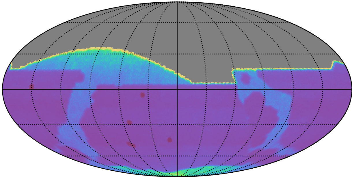
too_elab_r8_d2_gz_v3.4_10yrs All sky: Proper Motion Uncert @ 20.5
