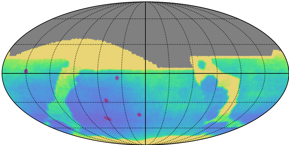
too_elab_r8_d2_gz_v3.4_10yrs All sky: Parallax Uncert @ 24.0
