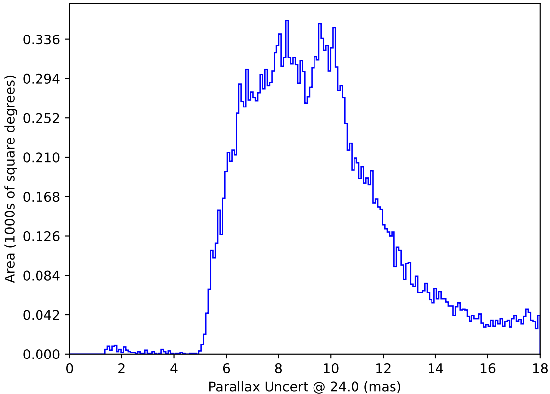
too_elab_r8_d2_gz_v3.4_10yrs All sky: Parallax Uncert @ 24.0
