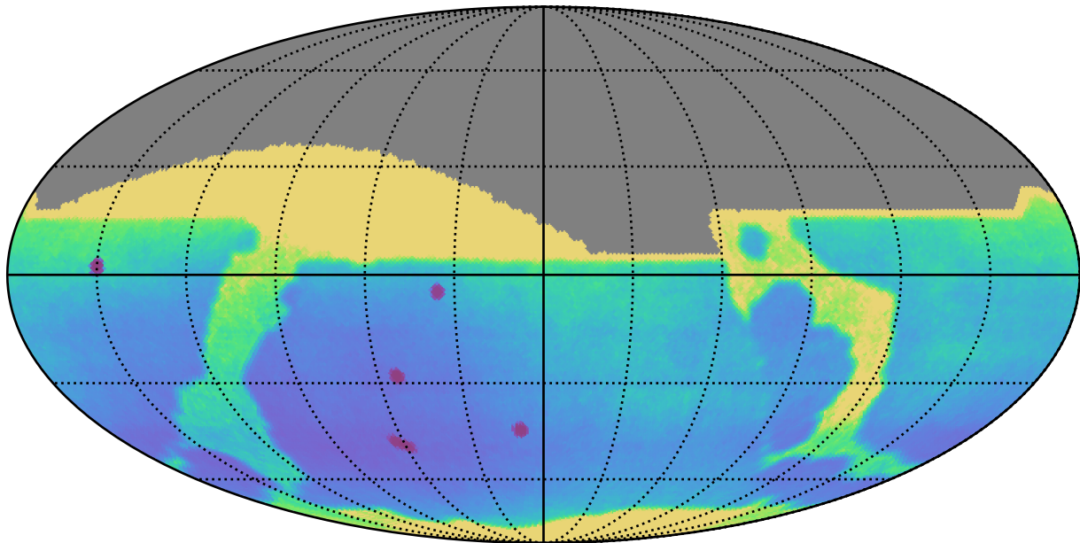
too_elab_r8_d2_gz_v3.4_10yrs All sky: Parallax Uncert @ 22.4
