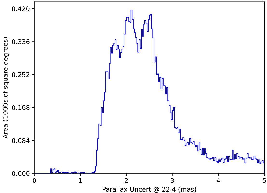
too_elab_r8_d2_gz_v3.4_10yrs All sky: Parallax Uncert @ 22.4
