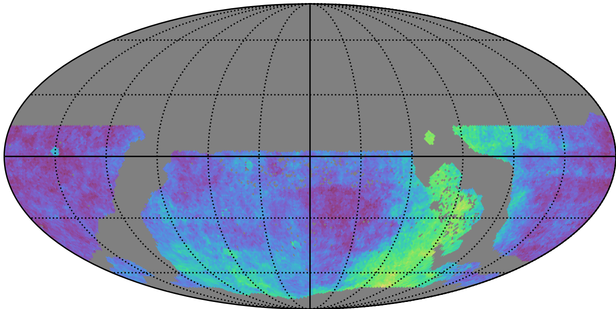
too_elab_r8_d2_gz_v3.4_10yrs WFD: Parallax Coverage @ 24.0
